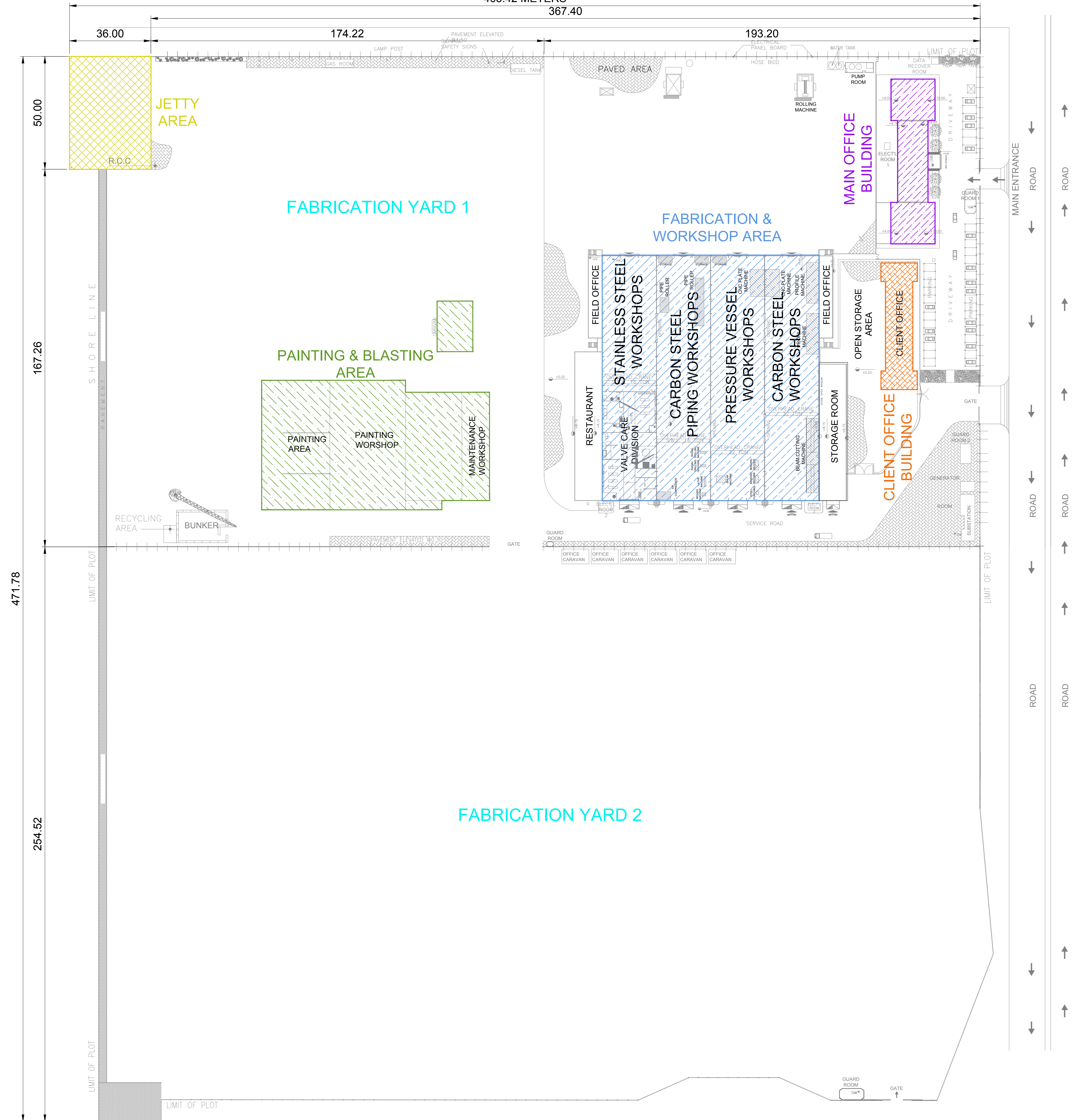
FABRICATION YARD LAYOUT PLAN
